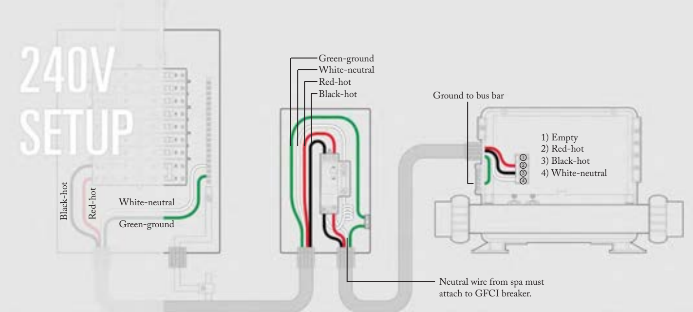
60Hz install (typical US/Canada)
