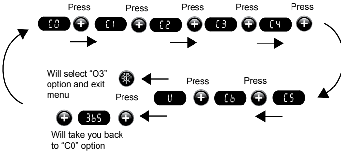
Figure 2: Menu for spas NOT equipped with a circulation pump.
